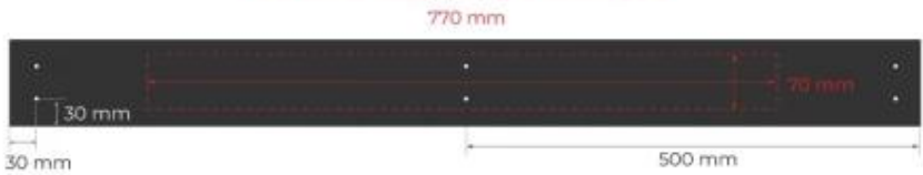
Top view with fixing points and burner cutout with lip in bottom plate
